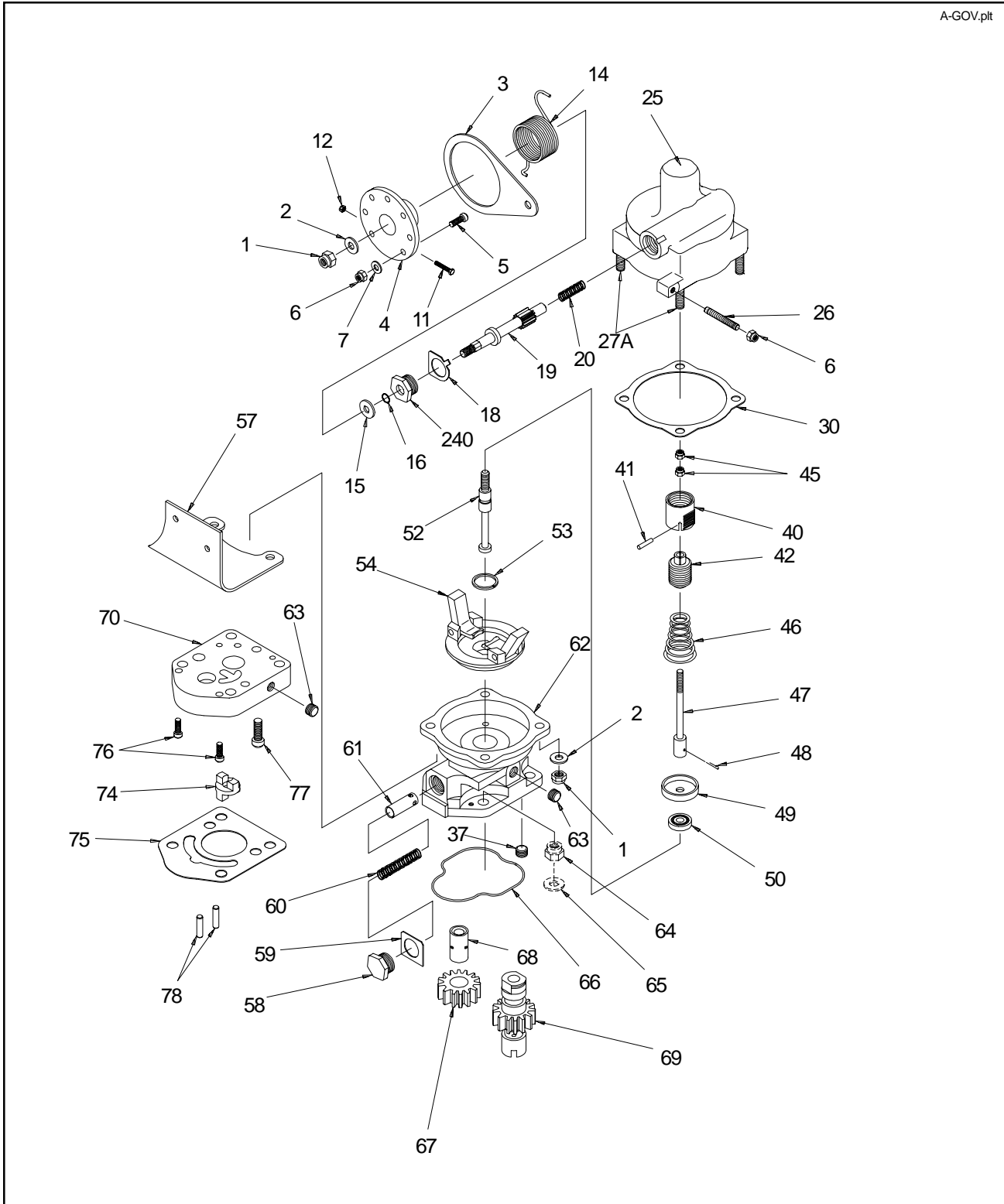
A Series Governor Assembly Figure 1001
